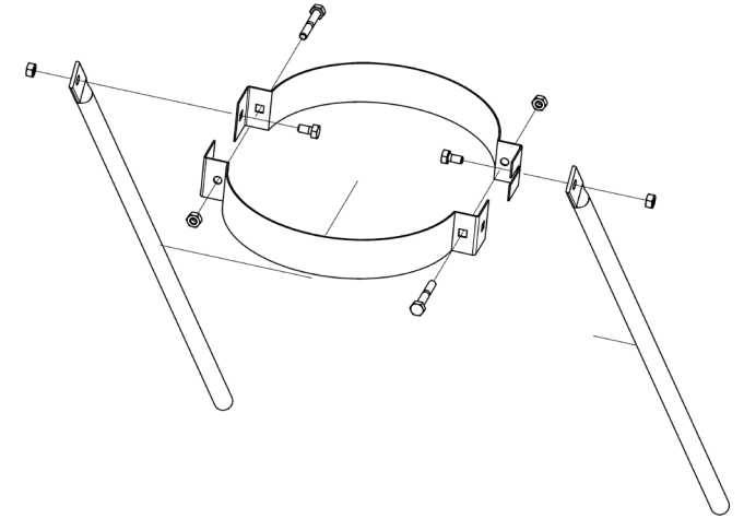
Figure 2 - Exploded View
