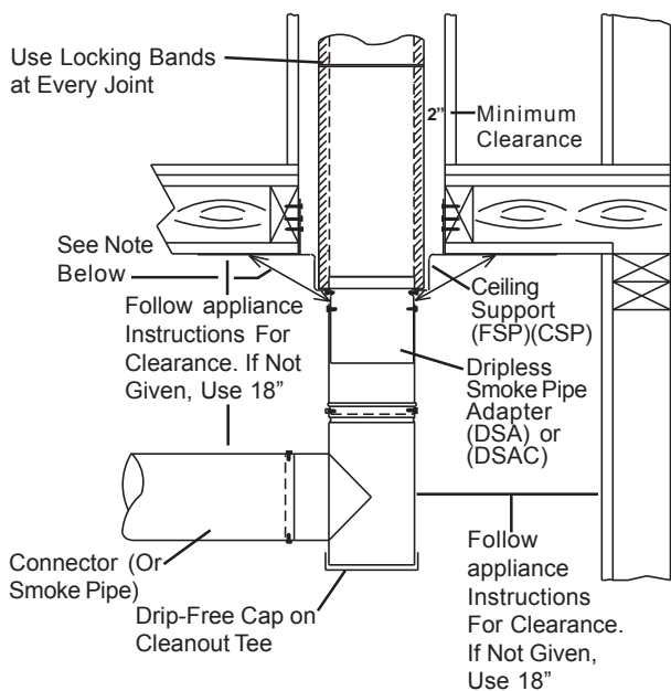
FIG. 3 CONNECTOR CLEARANCES
