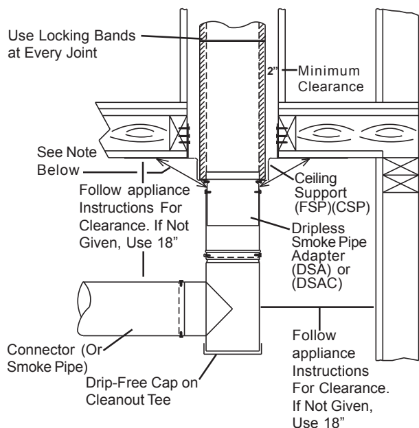
FIG. 3 CONNECTOR CLEARANCES
