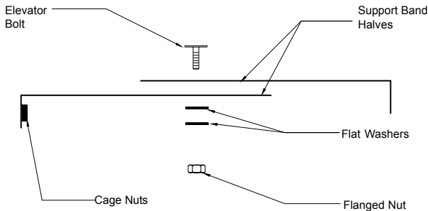
Topview assembly of Support Band - Figure 3 Elevator Bolt, Washers and Nut
